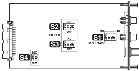
AD-20 component side (location of switches S1 - S4)
